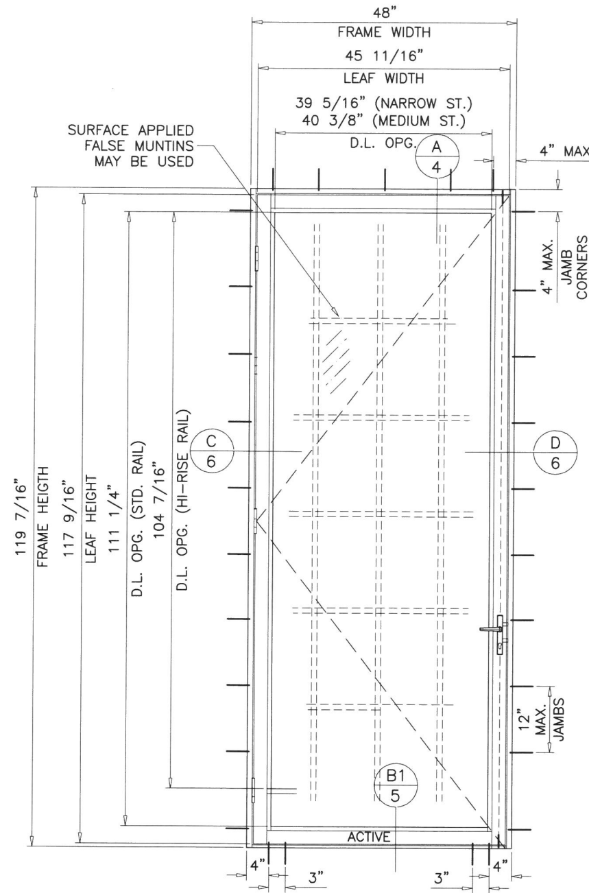
TYPICAL ELEVATION ( X ) COMMERCIAL SILL
